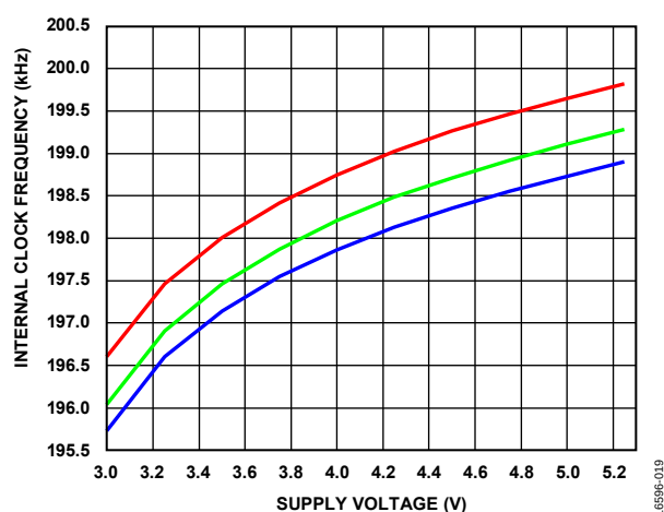
Figure 19. Internal Clock Frequency vs. Supply Voltage at 25°C
