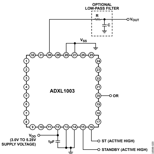
Figure 20. Application Circuit
