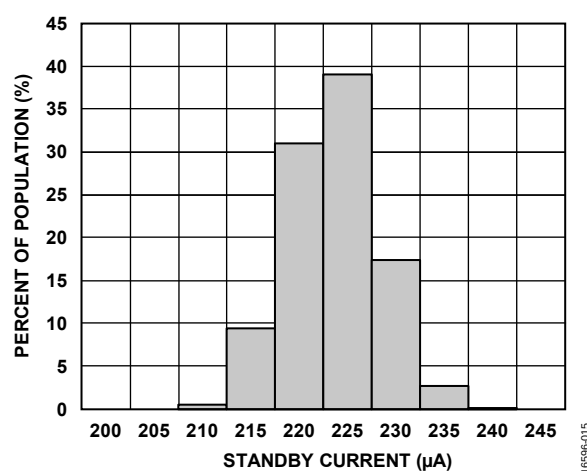
Figure 15. Standby Current Histogram at 25°C
