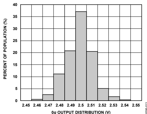
Figure 13. 0g Offset Histogram at 25°C
