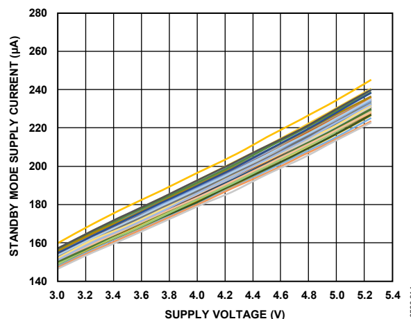
Figure 14. Standby Current vs. Supply Voltage
